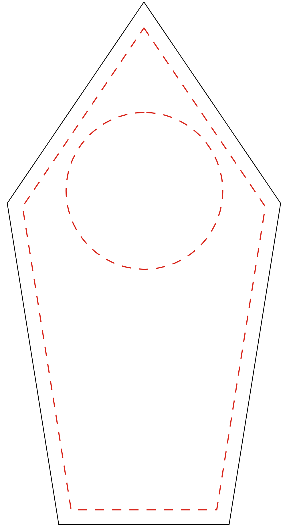
Job Name - Job # - C0555C - 9½" x 5" x ¾" Clear Acrylic Laser Imprint Area 4.375" x 8.75" (Red Dotted Lines)
